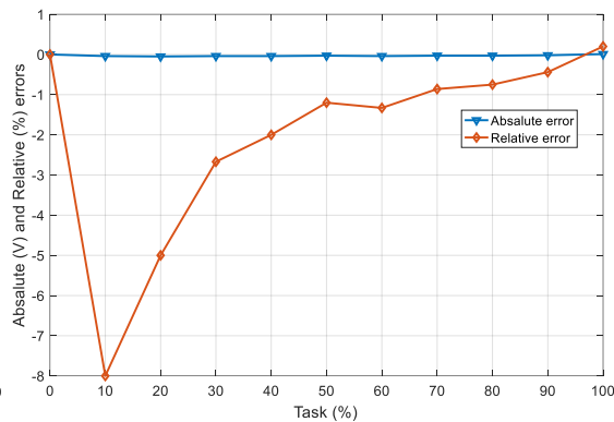
Figure 7. The error of output signal versus voltage
